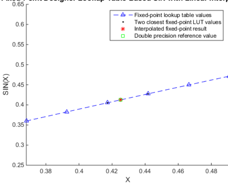
Fixed-Point Designer Lookup Table Based SIN with Linear Interpolation
