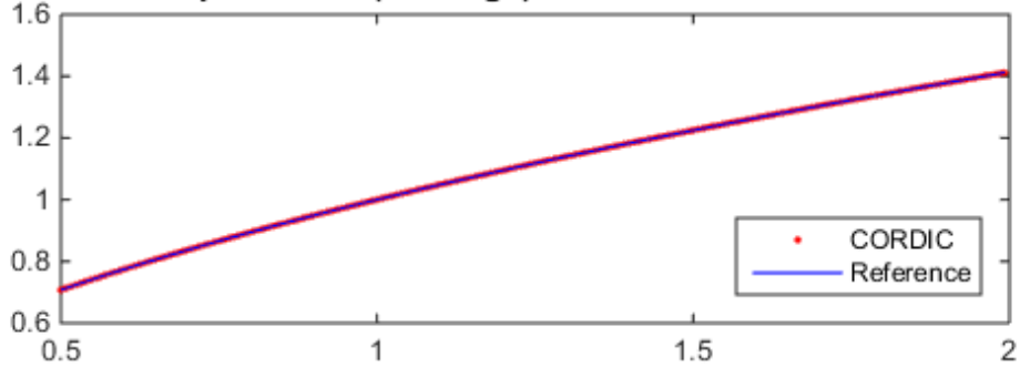
CORDIC Square Root (In-Range) and MATLAB Reference Results
